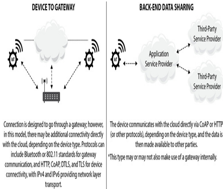
Figure 8-3 IoT communication models
