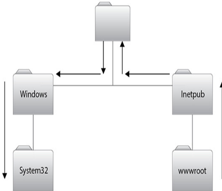
Figure 6-2 Directory traversal
