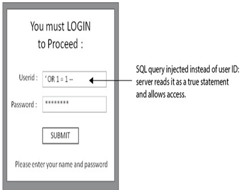
Figure 6-7 SQL injection
