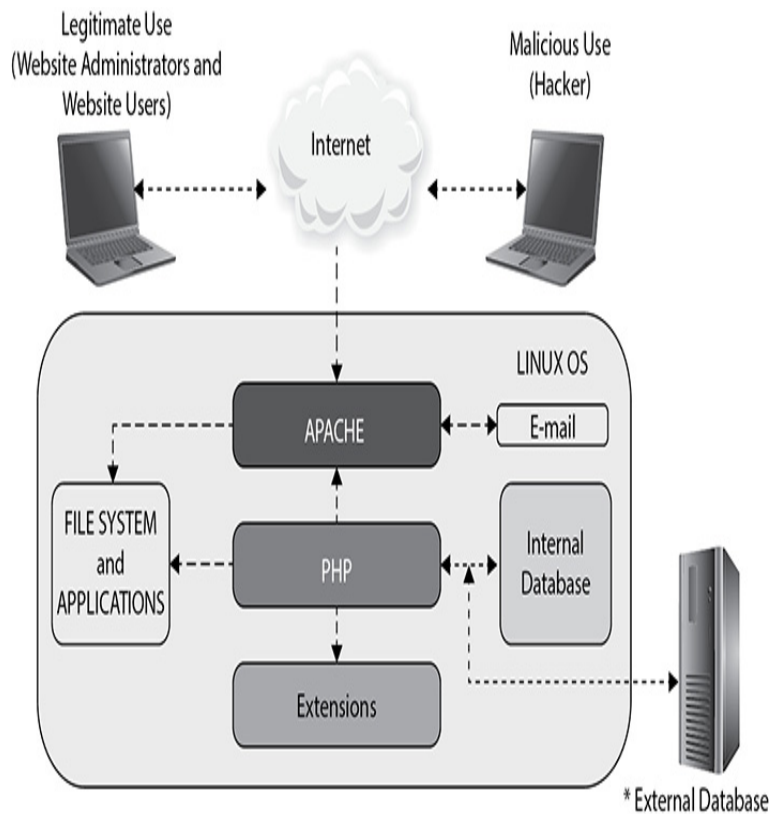
Figure 6-1 Apache
