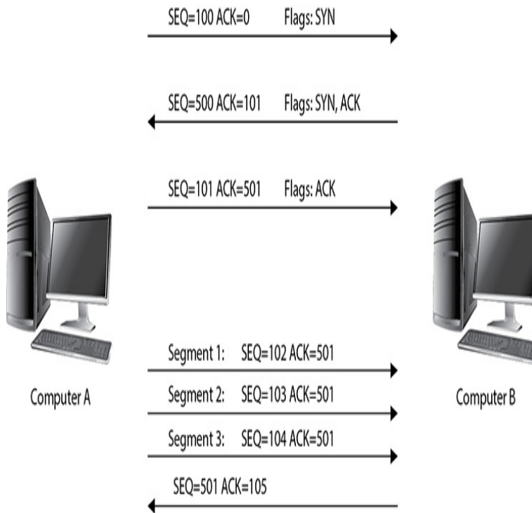
Figure 10-5 TCP communication
