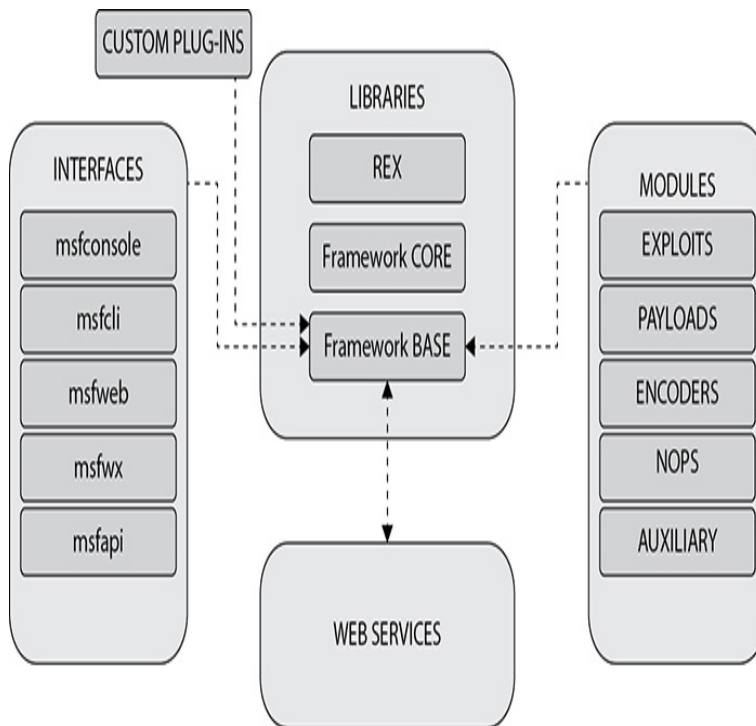
Figure 6-4 Metasploit
