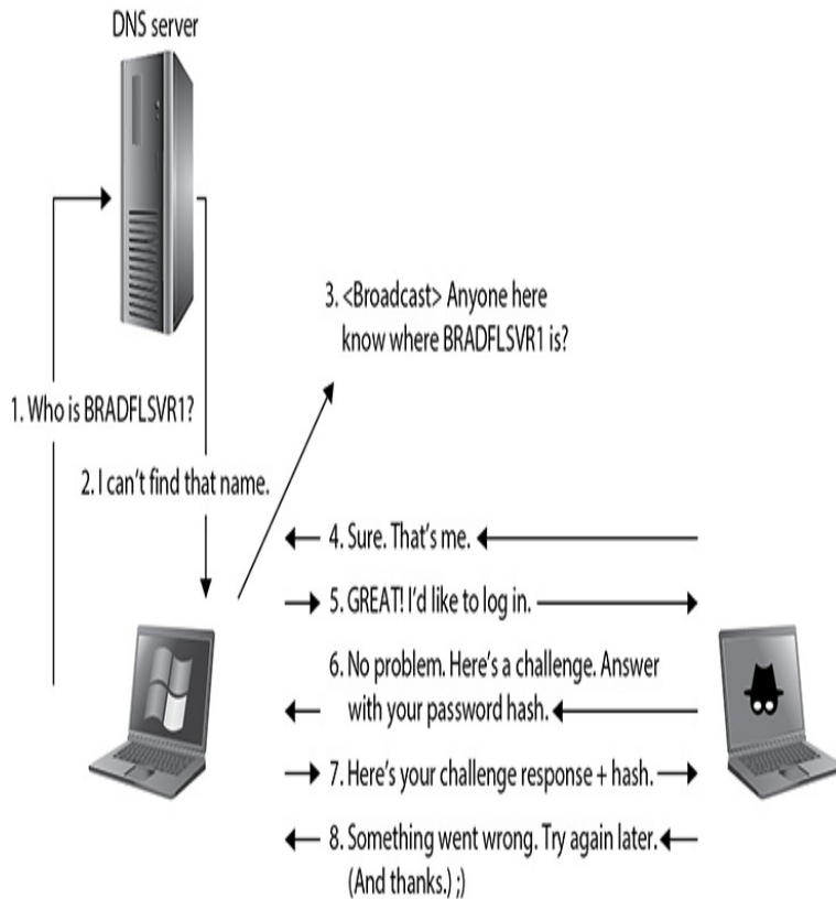
Figure 5-5 LLMNR attack
