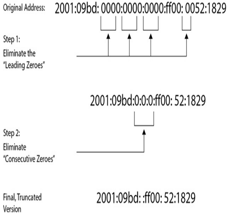
Figure 4-4 IPv6 address truncation
