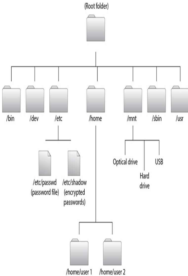
Figure 5-3 Linux file structure
