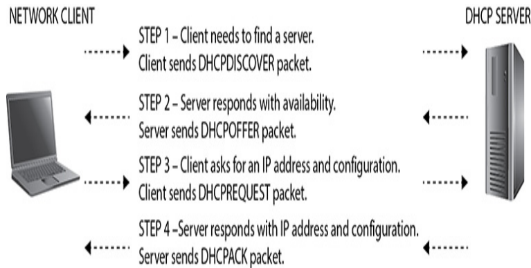
Figure 4-6 DHCP in action
