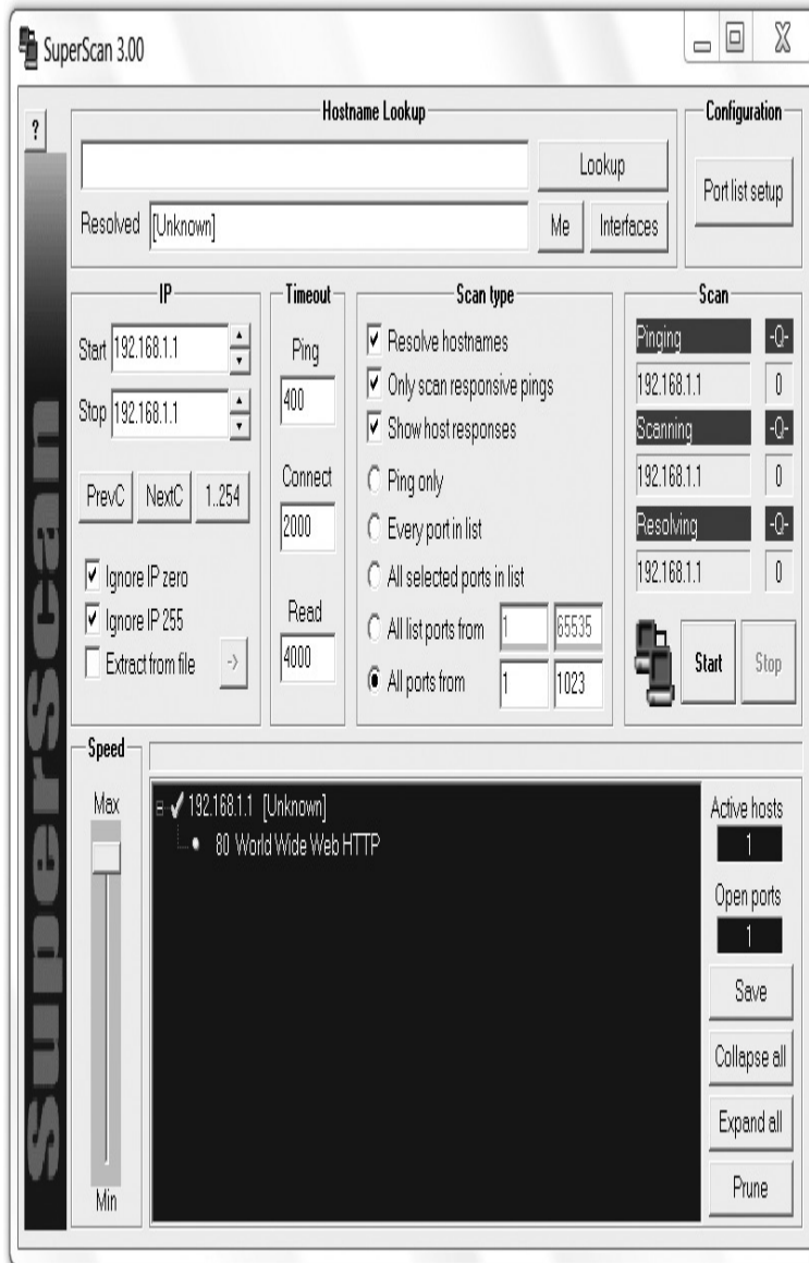
Figure 3-11 SuperScan
