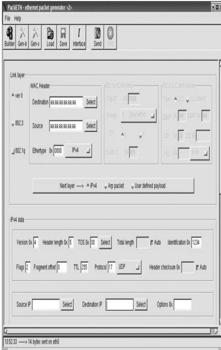
Figure 4-11 PackETH
