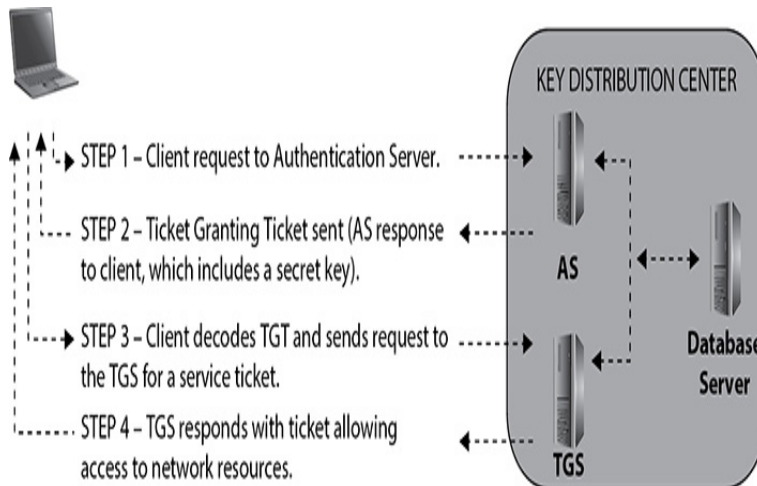
Figure 5-2 Kerberos in action
