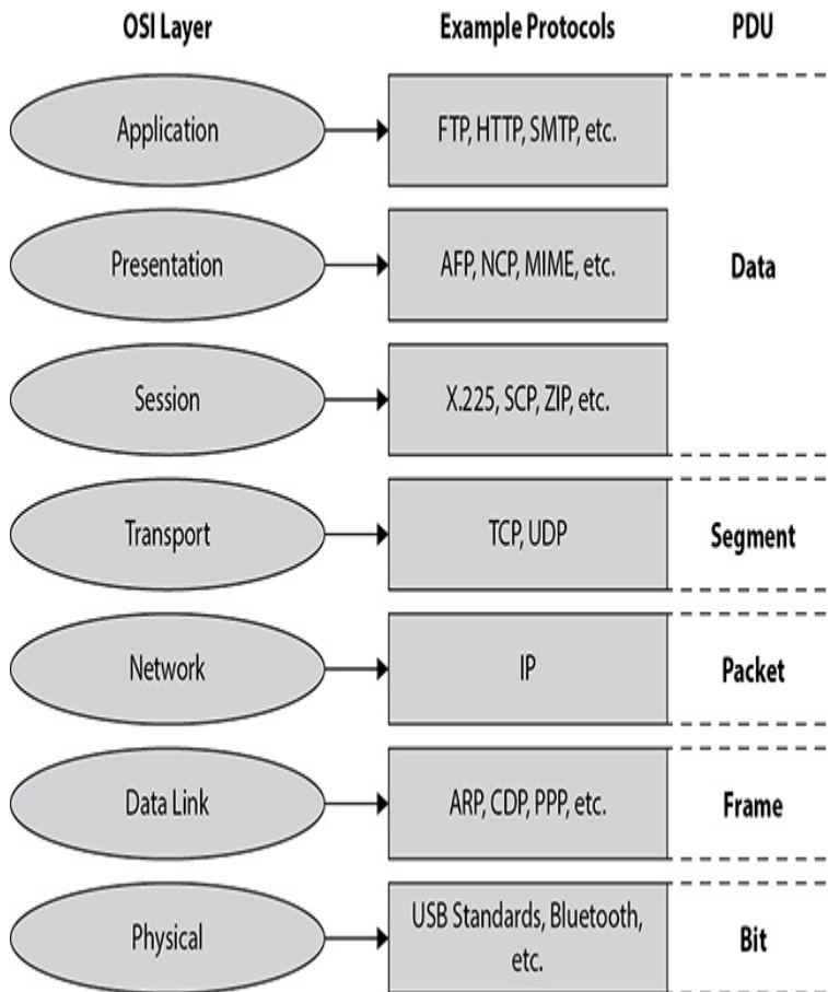
Figure 1-1 OSI reference model
