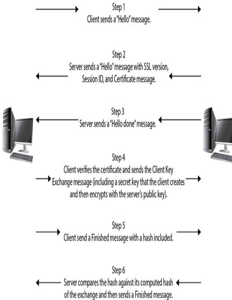
Figure 11-3 SSL connection steps
