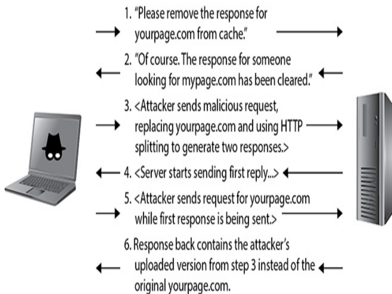
Figure 6-3 Web cache poisoning
