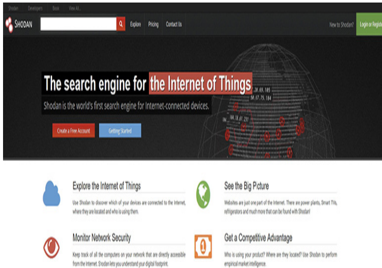
Figure 8-4 Shodan
