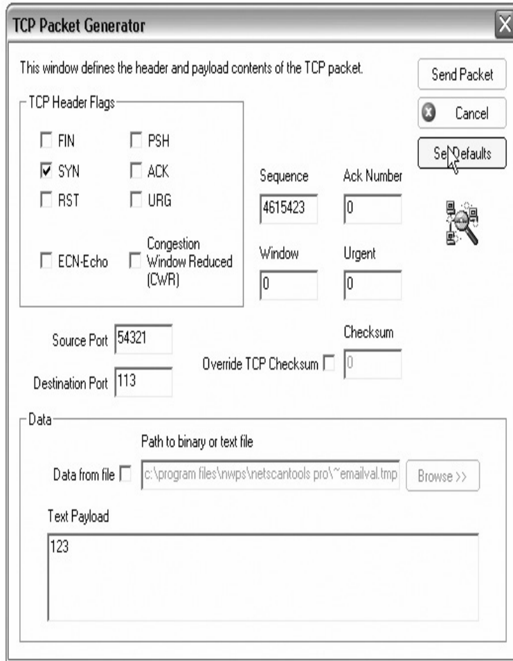
Figure 4-10 Packet Generator
