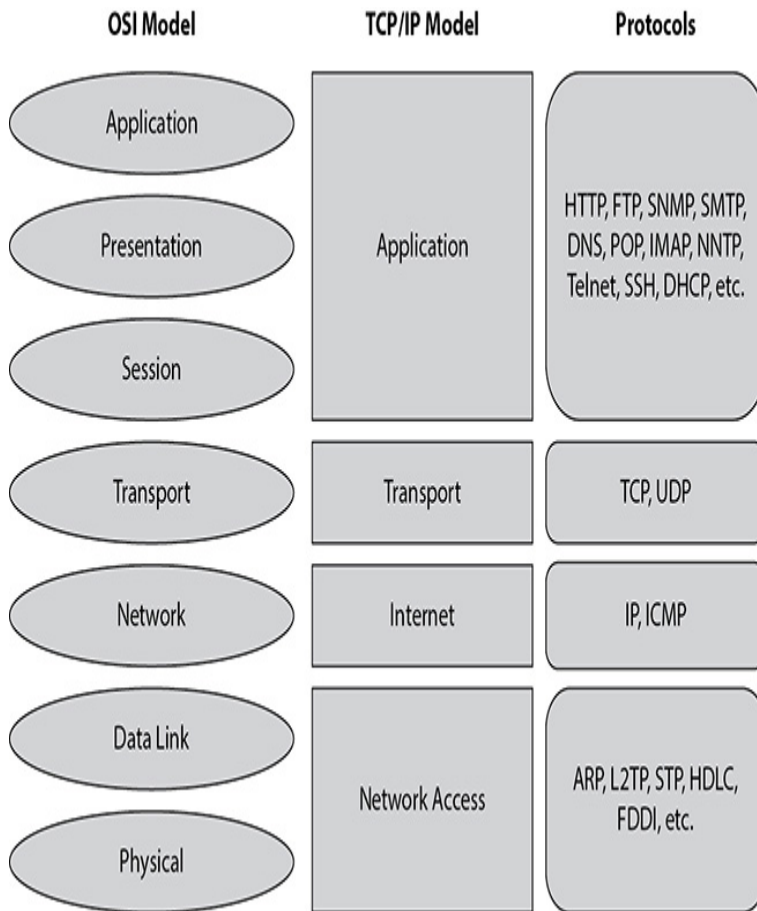
Figure 1-2 TCP/IP stack
