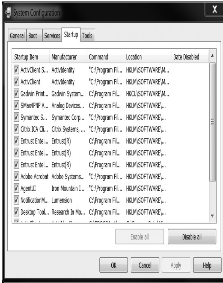
Figure 10-3 msconfig
