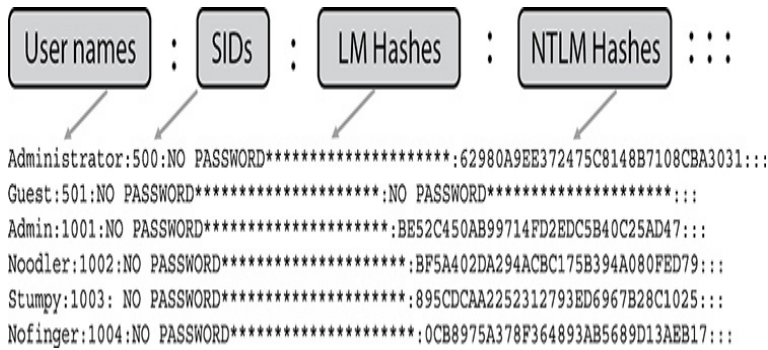
Figure 5-1 SAM file
