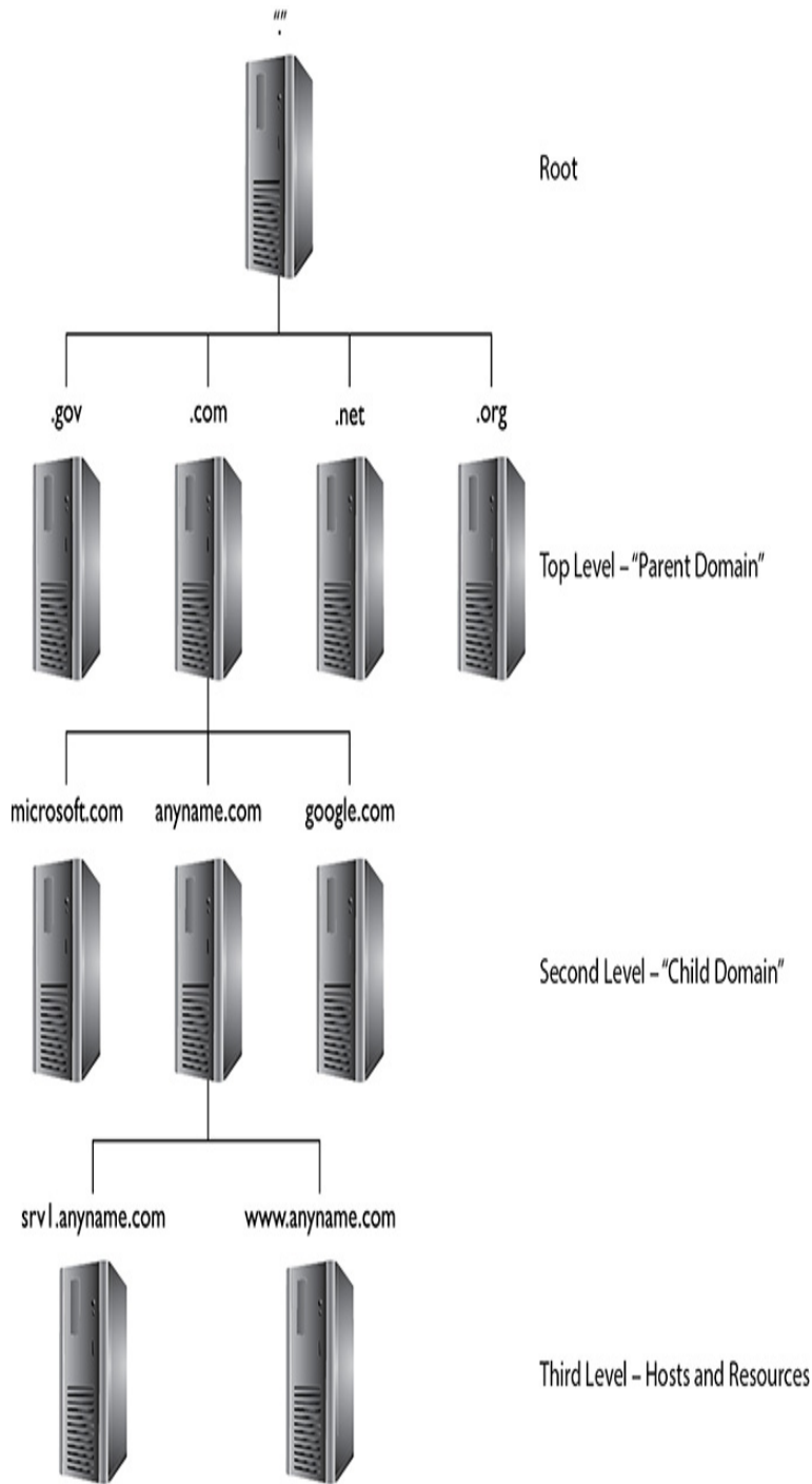
Figure 2-4 DNS structure
