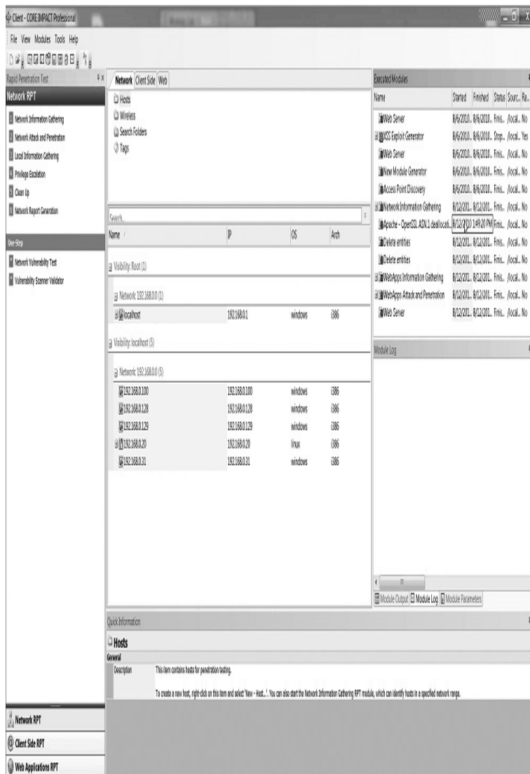
Figure 13-2 Core Impact
