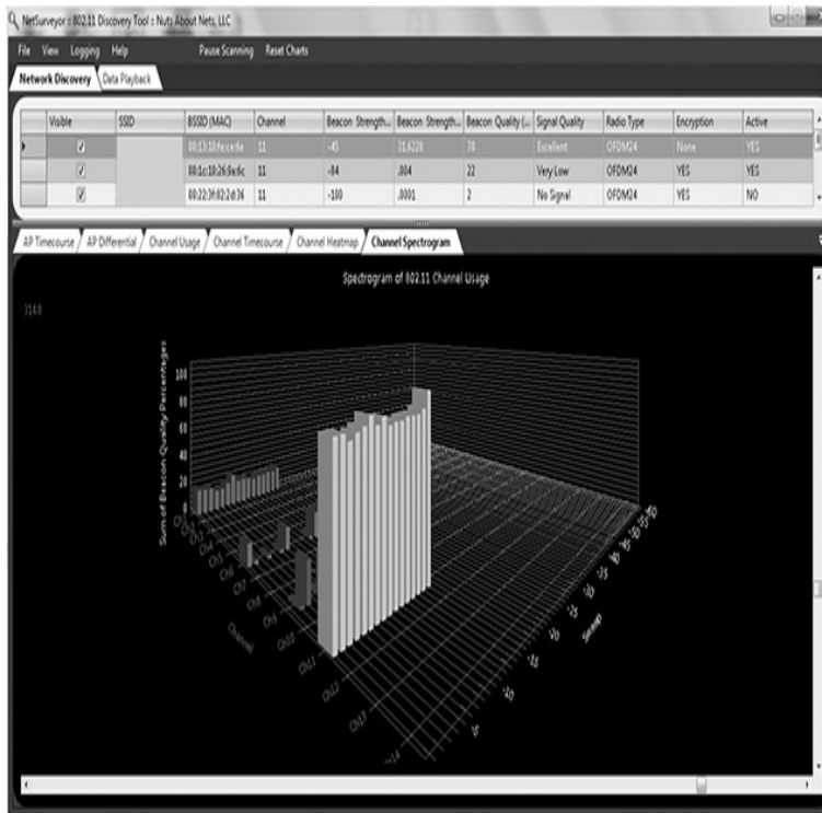
Figure 7-5 NetSurveyor
