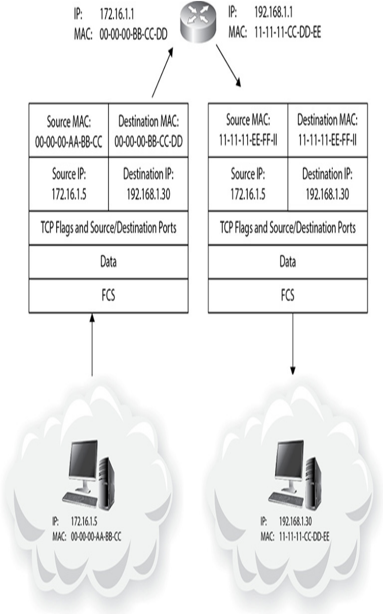
Figure 1-4 Ethernet frames in transit
