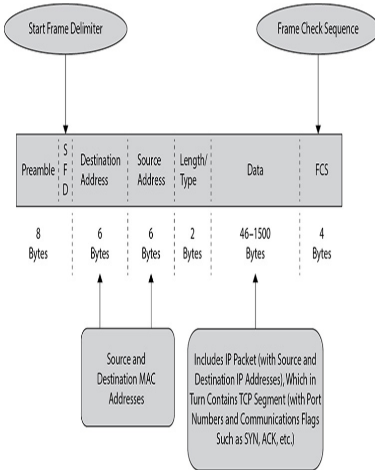
Figure 1-3 An Ethernet frame
