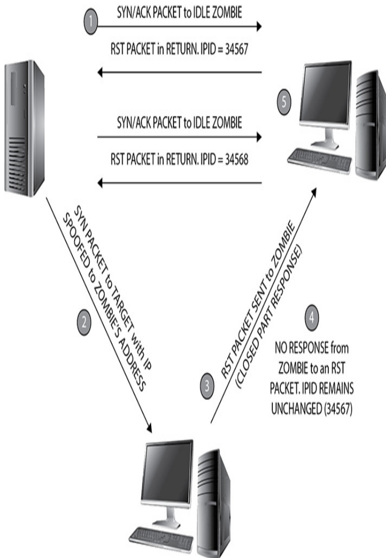
Figure 3-9 IDLE scanning: port closed
