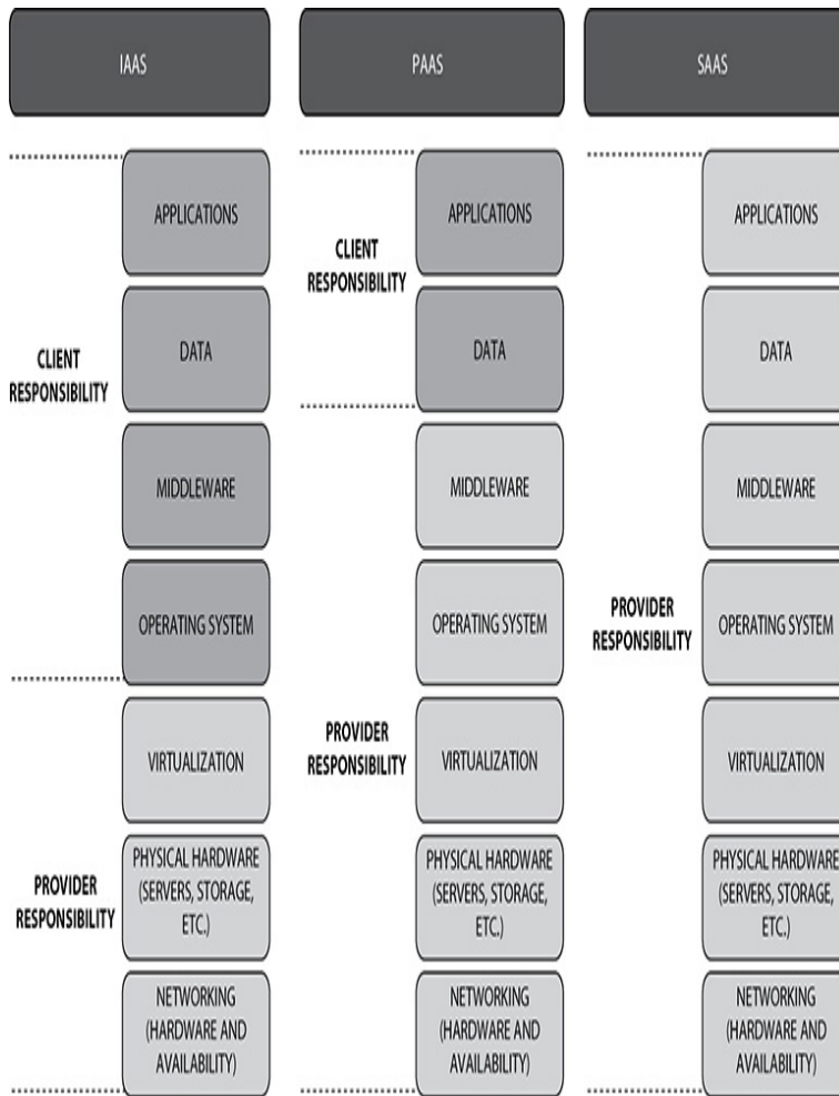
Figure 9-1 Cloud security alliance models
