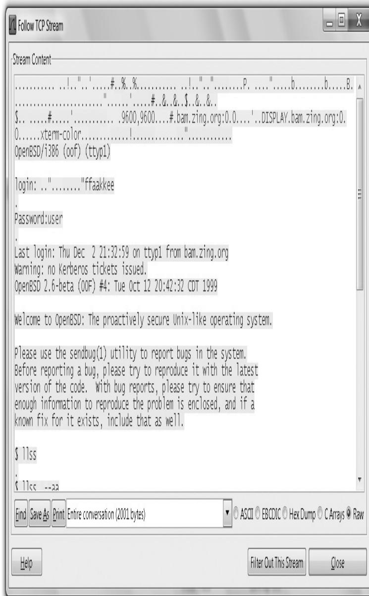
Figure 4-7 Telnet session in Wireshark
