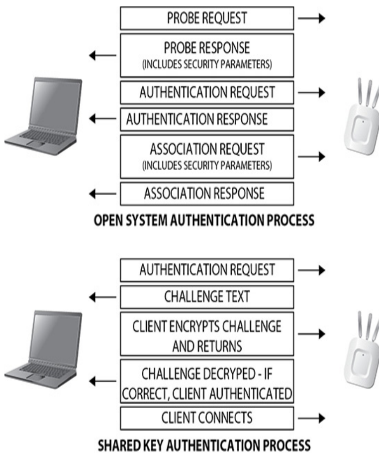
Figure 7-2 Wireless authentication methods
