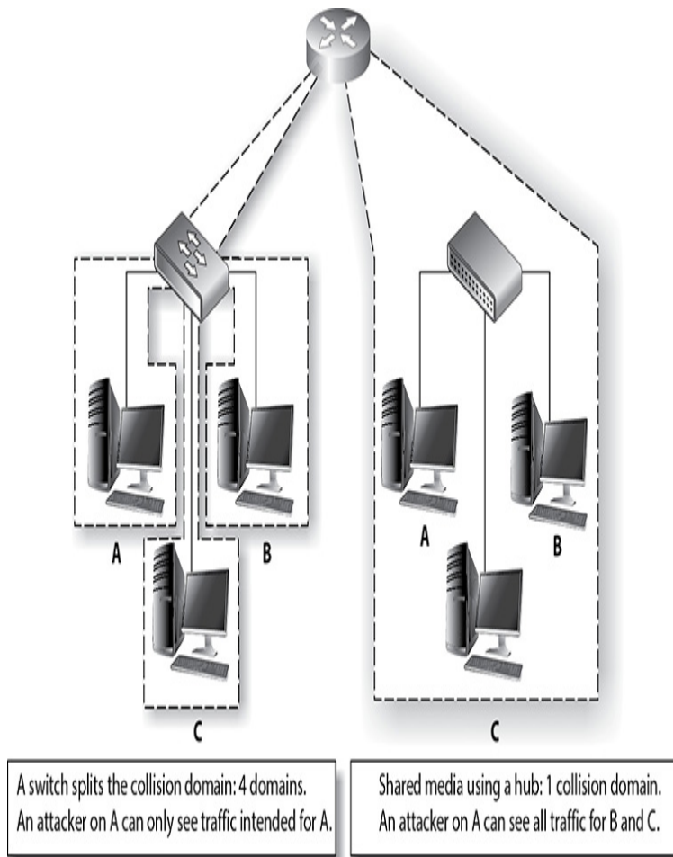
Figure 4-1 Collision domains and sniffing
