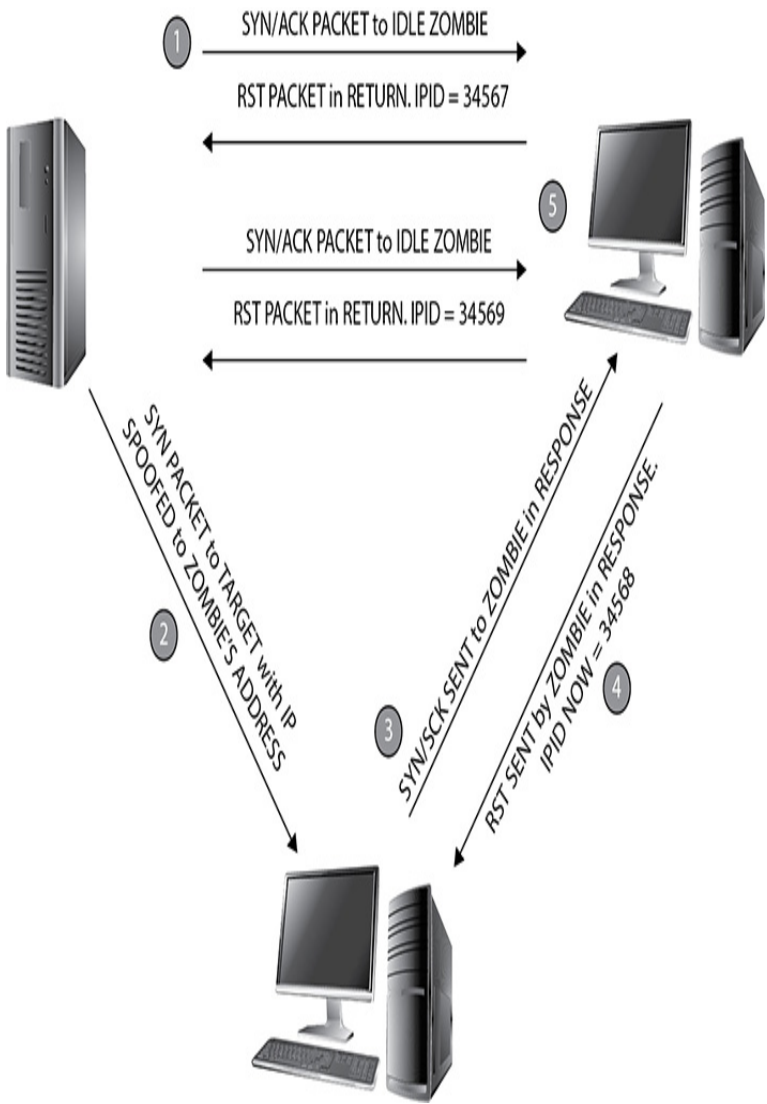
Figure 3-8 IDLE scanning: port open
