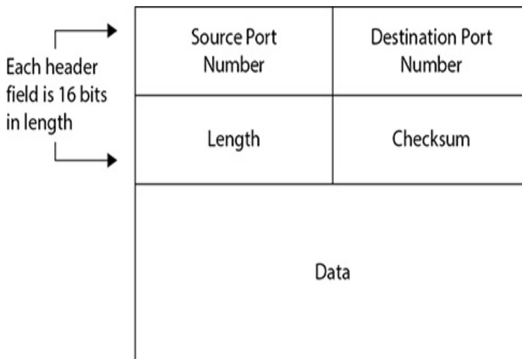
Figure 3-1 UDP datagram structure
