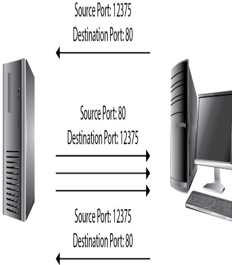
Figure 3-5 Port numbers in use
