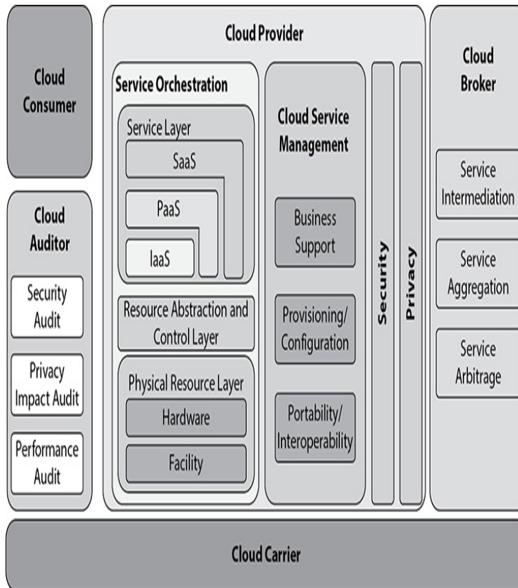
Figure 9-2 NIST Cloud Computing Reference Architecture
