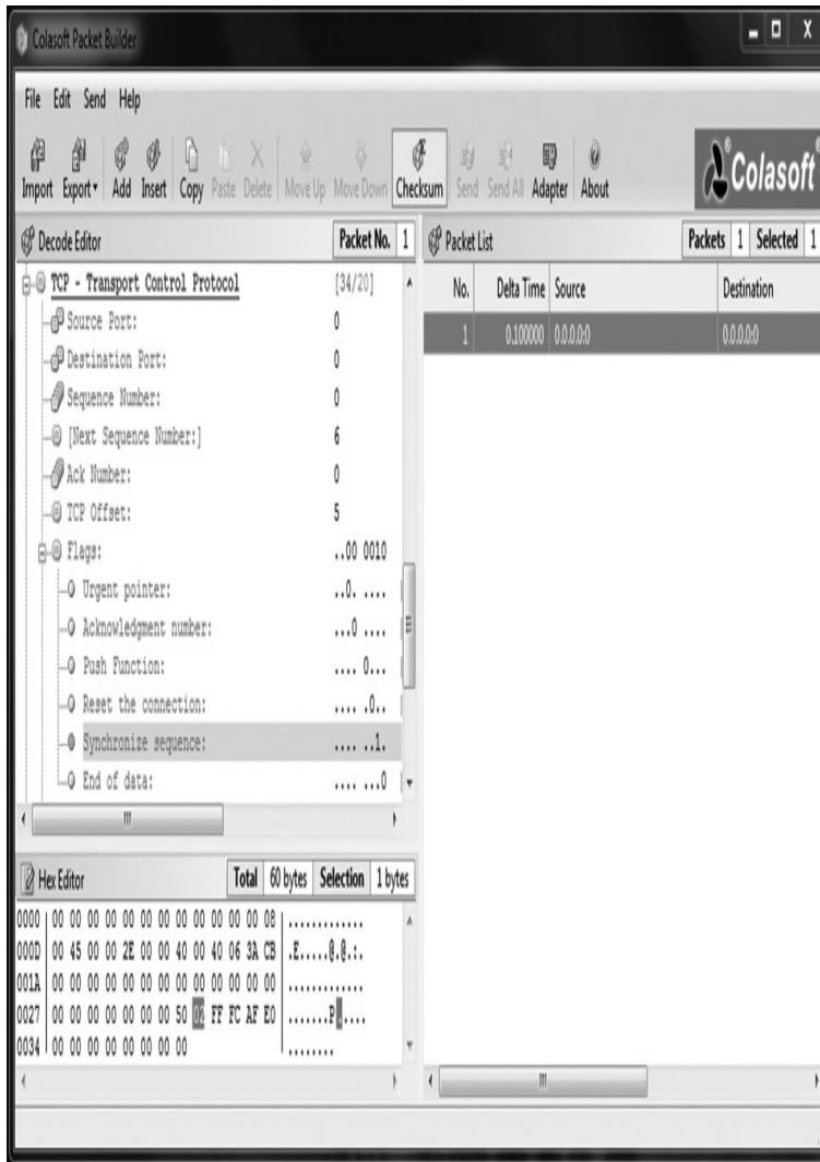
Figure 3-4 Colasoft Packet Builder
