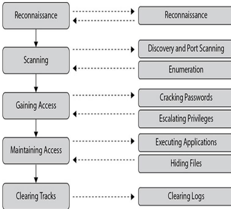
Figure 5-4 System attack phases
