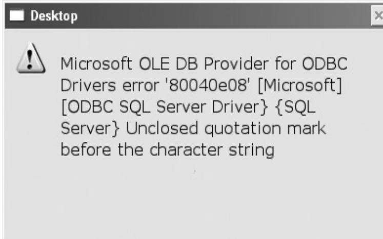
Figure 6-8 SQL error message
