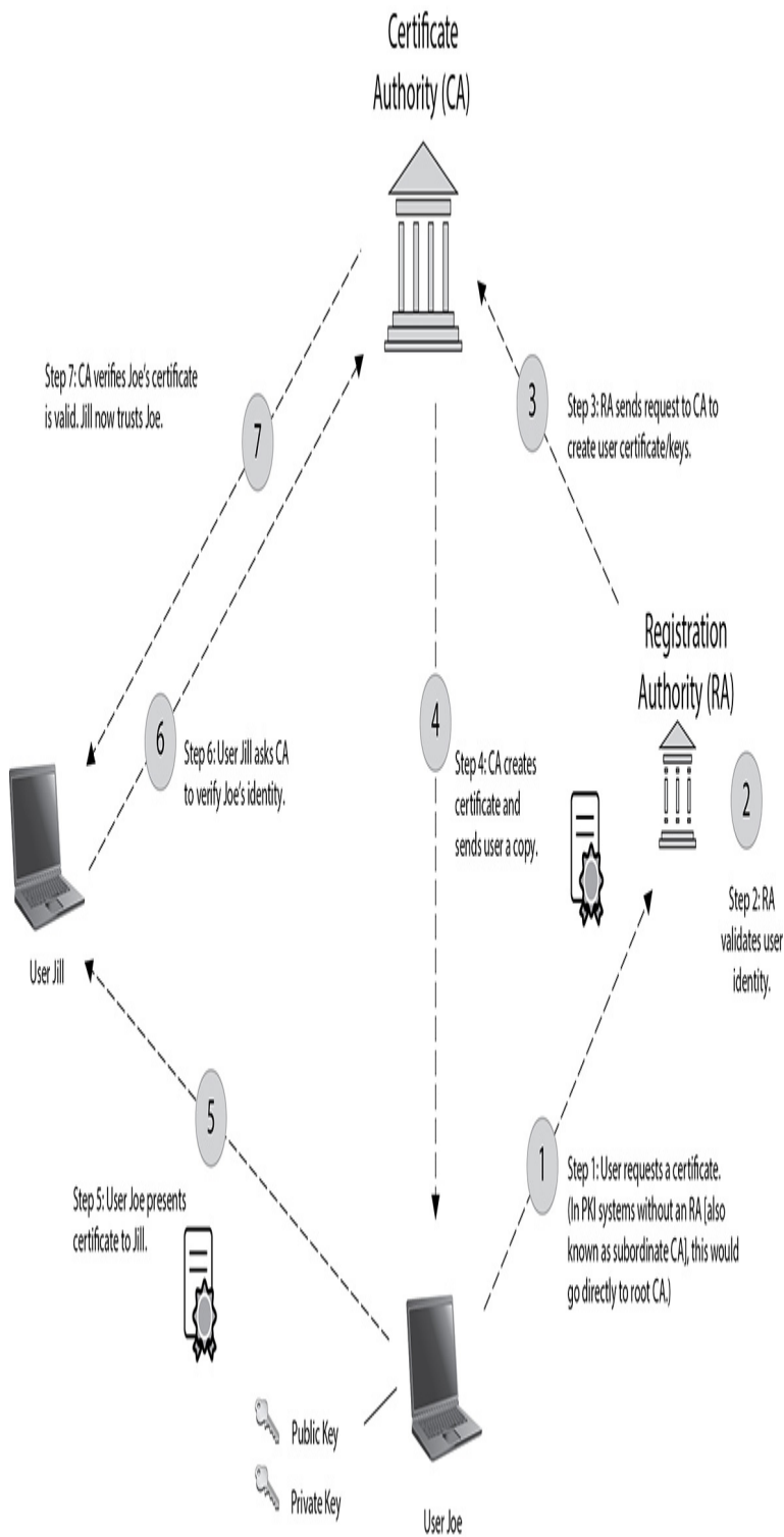
Figure 11-2 The PKI system
