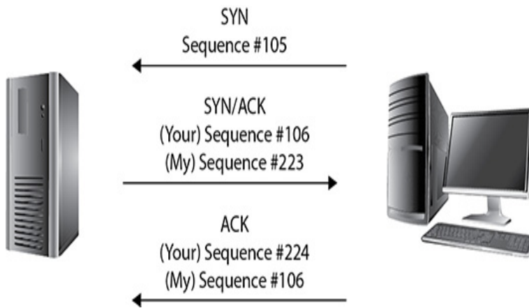
Figure 3-3 The three-way handshake
