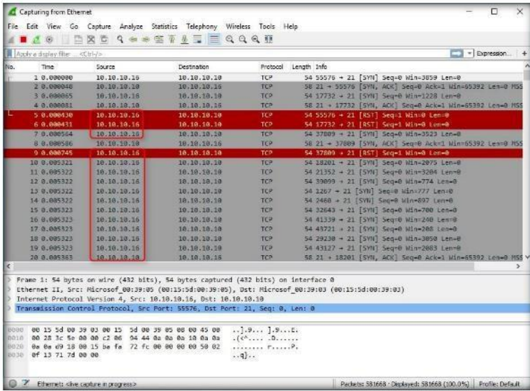
FIGURE 1.8: Analyzing the Traffic
