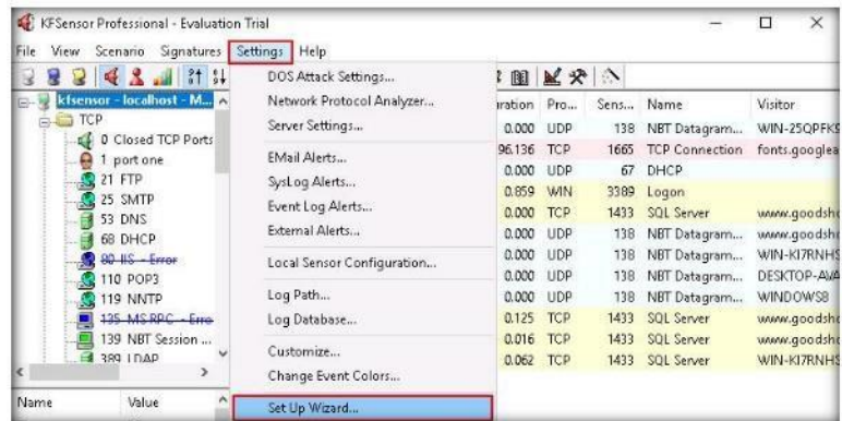
FIGURE 4.5: Launching KFSensor Set Up Wizard...
