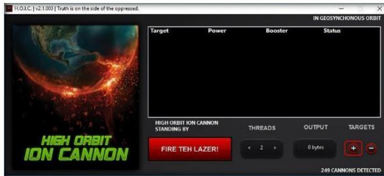
FIGURE 3.1: HOIC GUI
