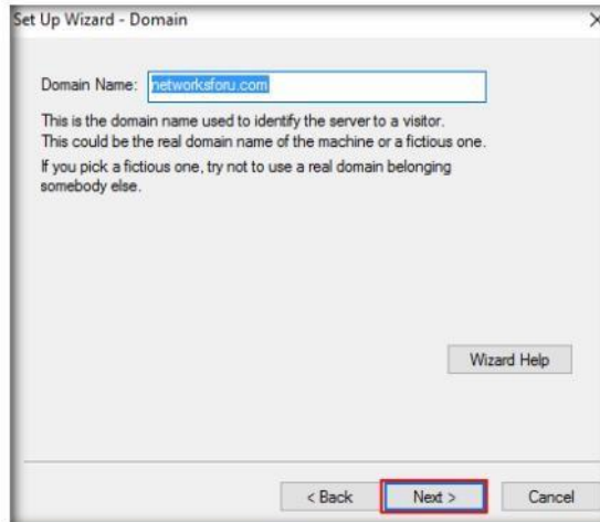
FIGURE 4.9: Domain wizard
