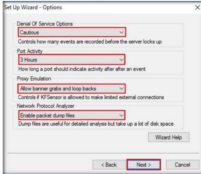
FIGURE 4.11: Options Wizard
