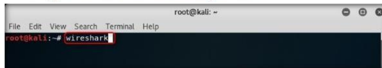
FIGURE 3.5: Launching Wireshark
