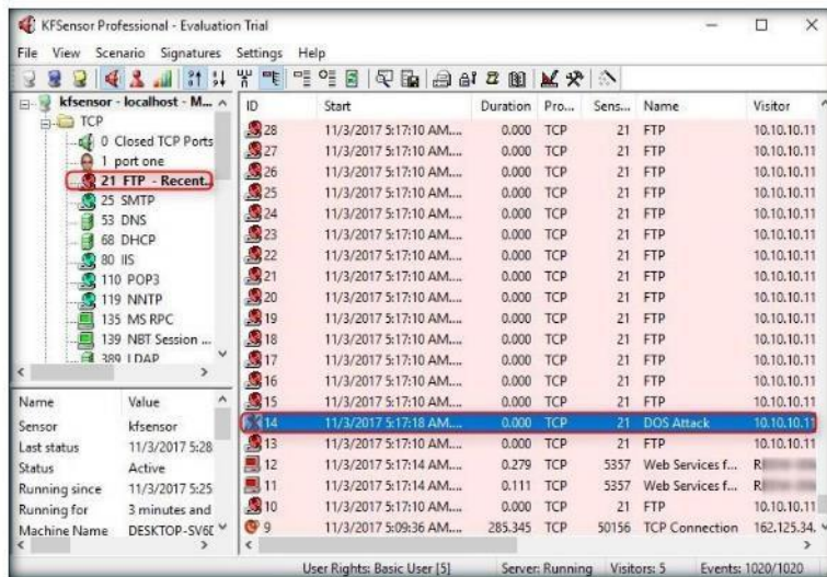
FIGURE 4.20: FTP Section Flooded with DOS Attack Events
