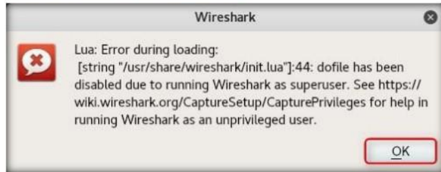
FIGURE 3.6: Error pop-up
