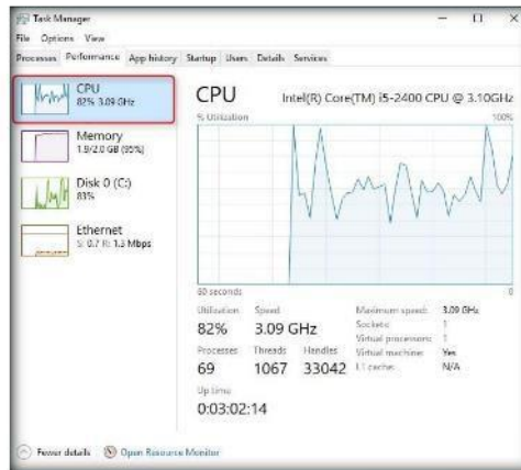
FIGURE 1.9: Analyzing the Machine's Performance
