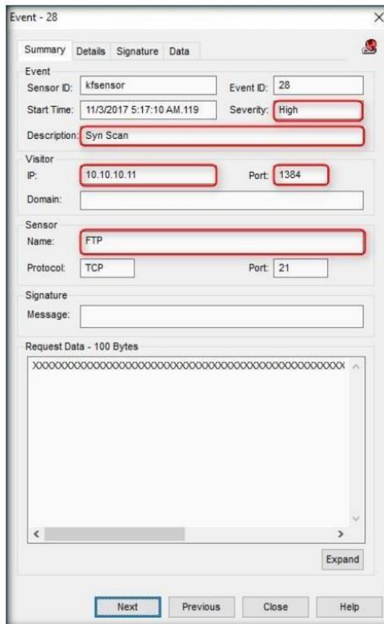
FIGURE 4.22: Viewing the Event Details
