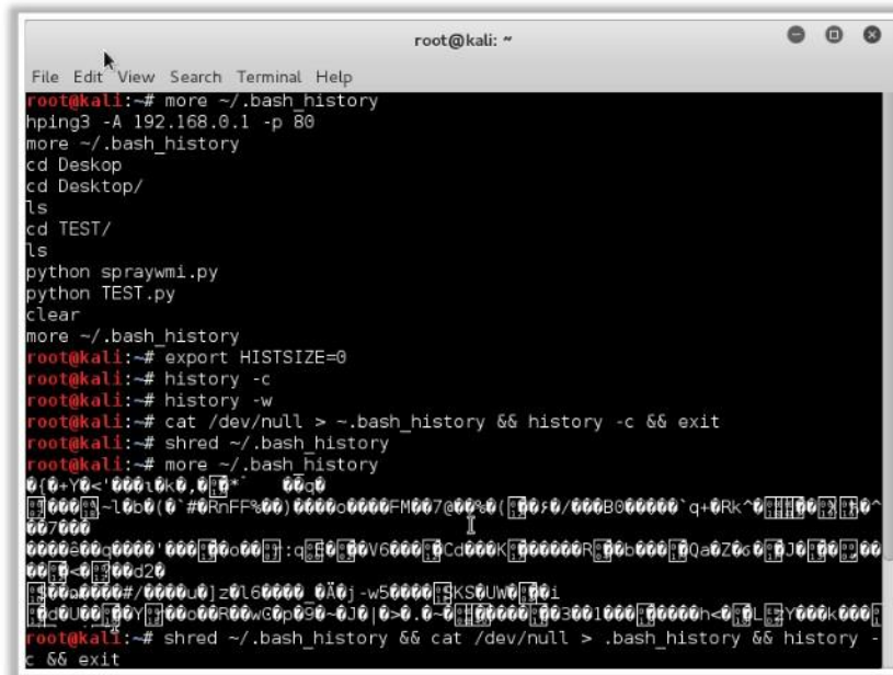
FIGURE 6.10: Covering BASH Shell tracks
