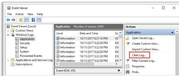
FIGURE 6.8: Clearing Event logs for Windows
