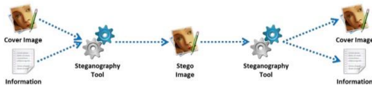
FIGURE 6.4: Image steganography process
