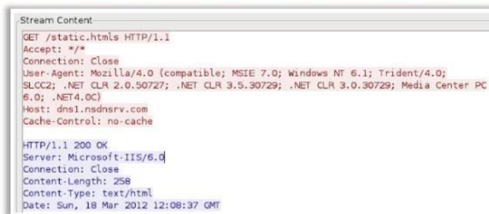
FIGURE 7.14: Screenshot displaying the requests sent to C&C Server for downloading static.htmls files
