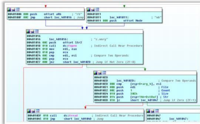
FIGURE 7.25: Screenshot displaying the extraction of c.wnry contents
