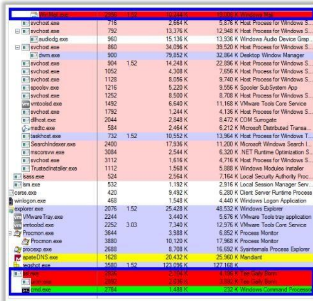
FIGURE 7.11: Screenshot displaying processes in Process Explorer
