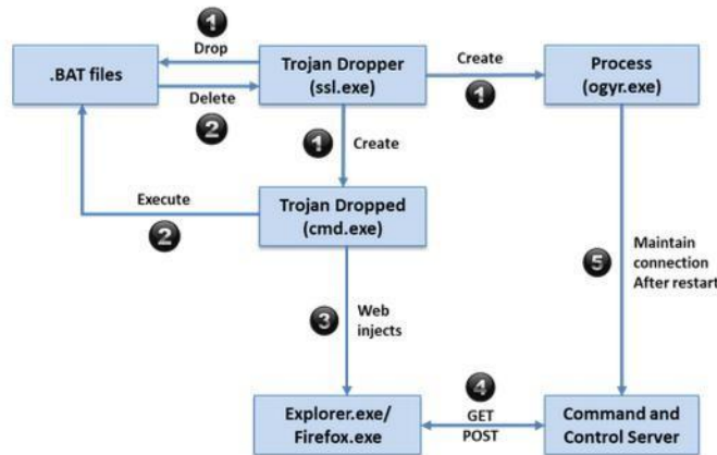
FIGURE 7.10: Screenshot displaying stages of Zeus Trojan attack
