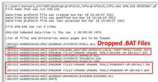
FIGURE 7.12: Screenshot displaying .BAT files location
