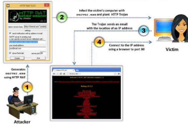
FIGURE 7.3: Working of HTTP RAT Trojan
