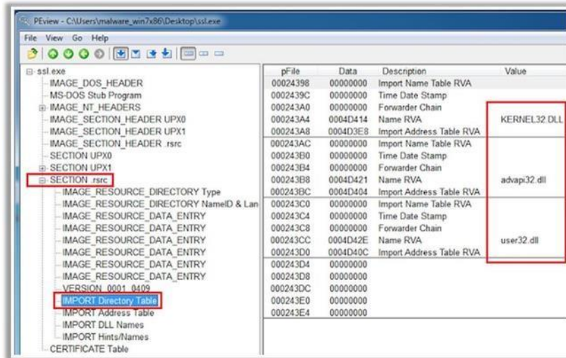
FIGURE 7.9: Screenshot displaying .dll files of Zeus Trojan
