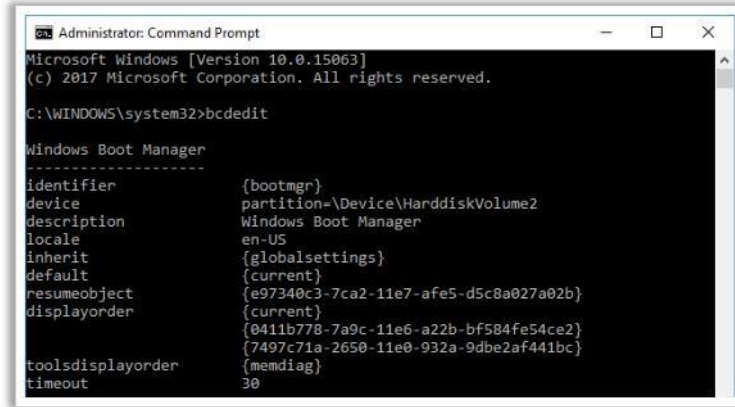
FIGURE 7.5: Screenshot displaying boot info
