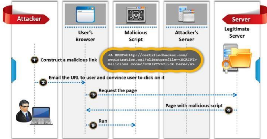
FIGURE 14.5: XSS example - attack via email
