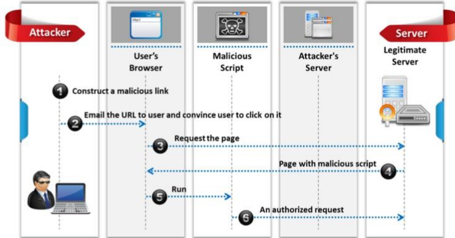
FIGURE 14.7: XSS example - Sending an unauthorized request
