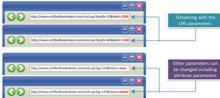
FIGURE 14.3: Parameter Tampering attack example
