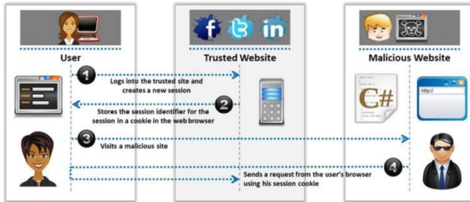
FIGURE 14.8: Cross-Site Request Forgery (CSRF) attack example
