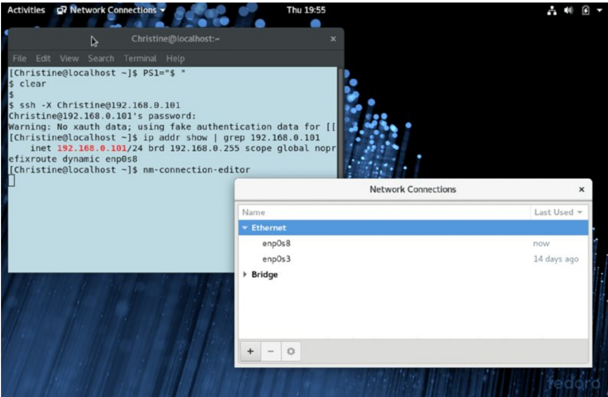
Figure 8.11 Forwarding X11
