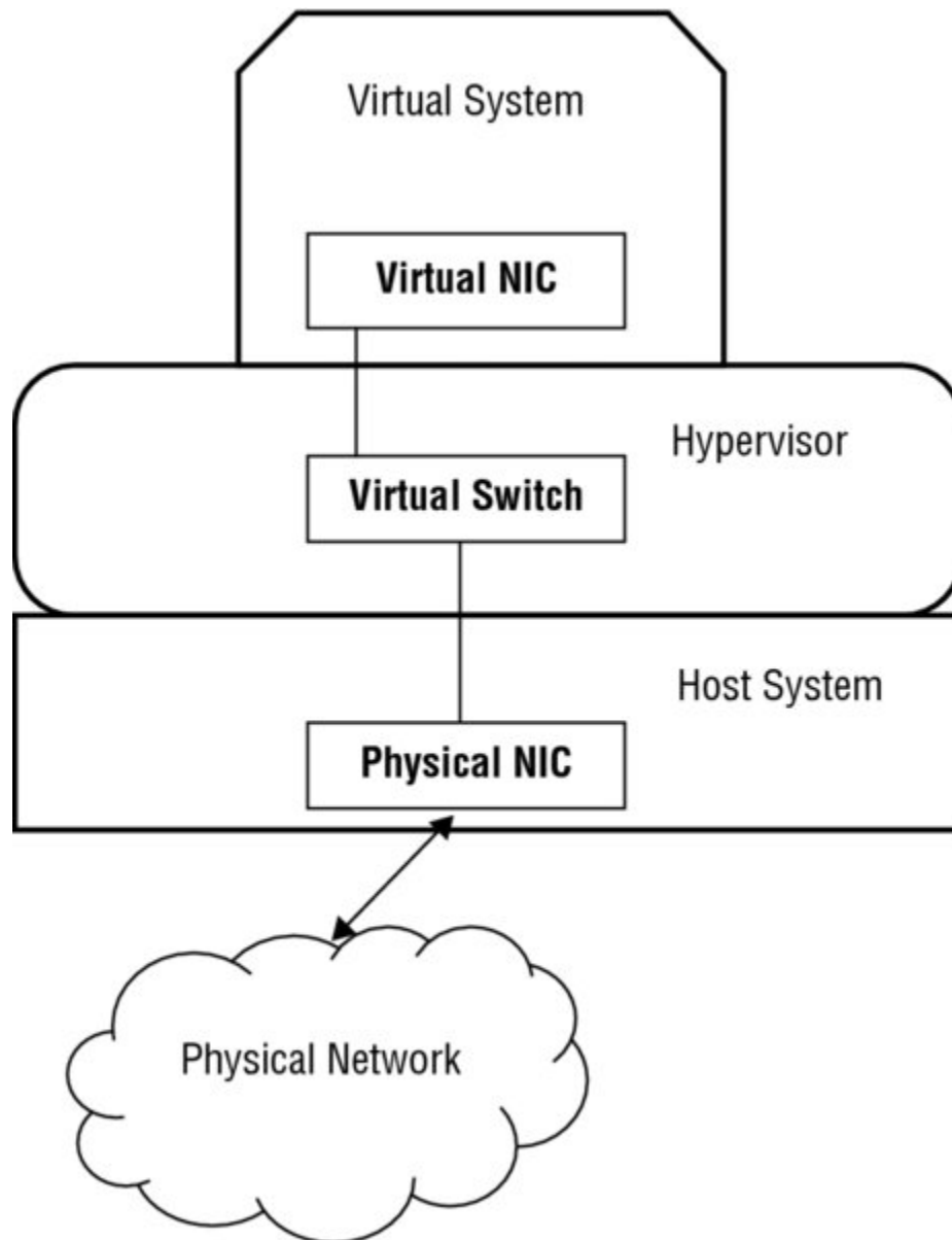
Figure 29.2 Virtual machine using a virtual switch
