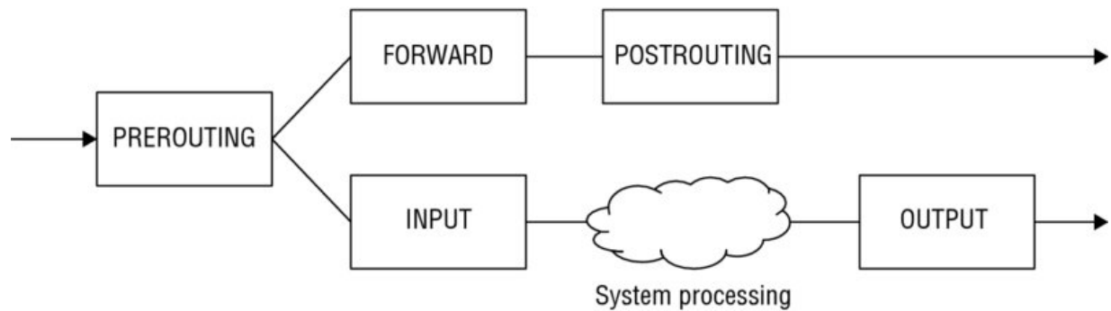
Figure 18.1 The packet processing chain
