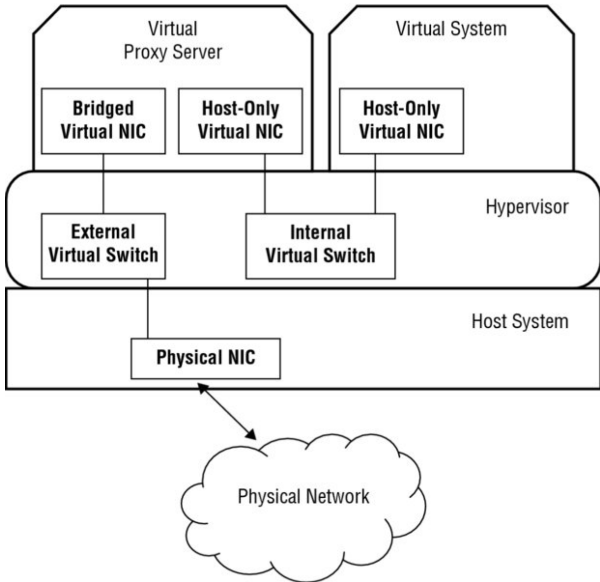
Figure 29.3 Virtual proxy server
