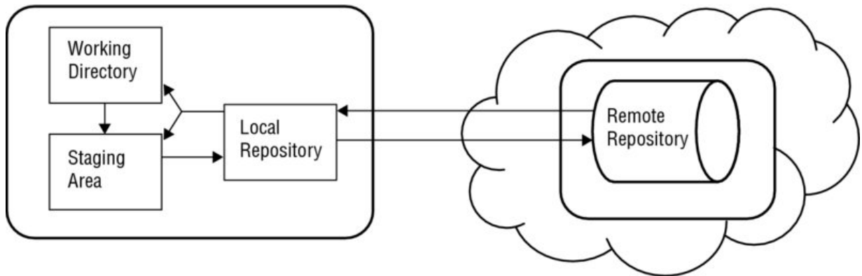
Figure 27.1 Conceptual depiction of the Git environment
