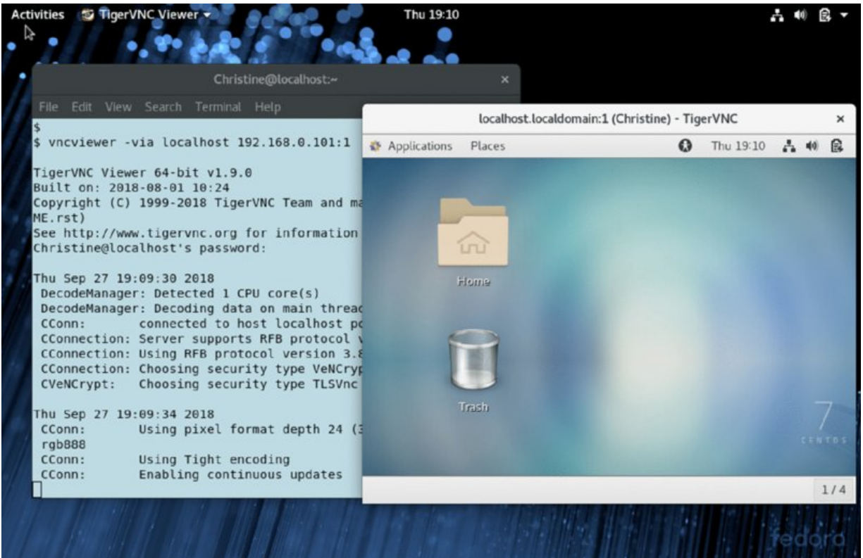
Figure 8.10 Using local SSH port forwarding with TigerVNC
