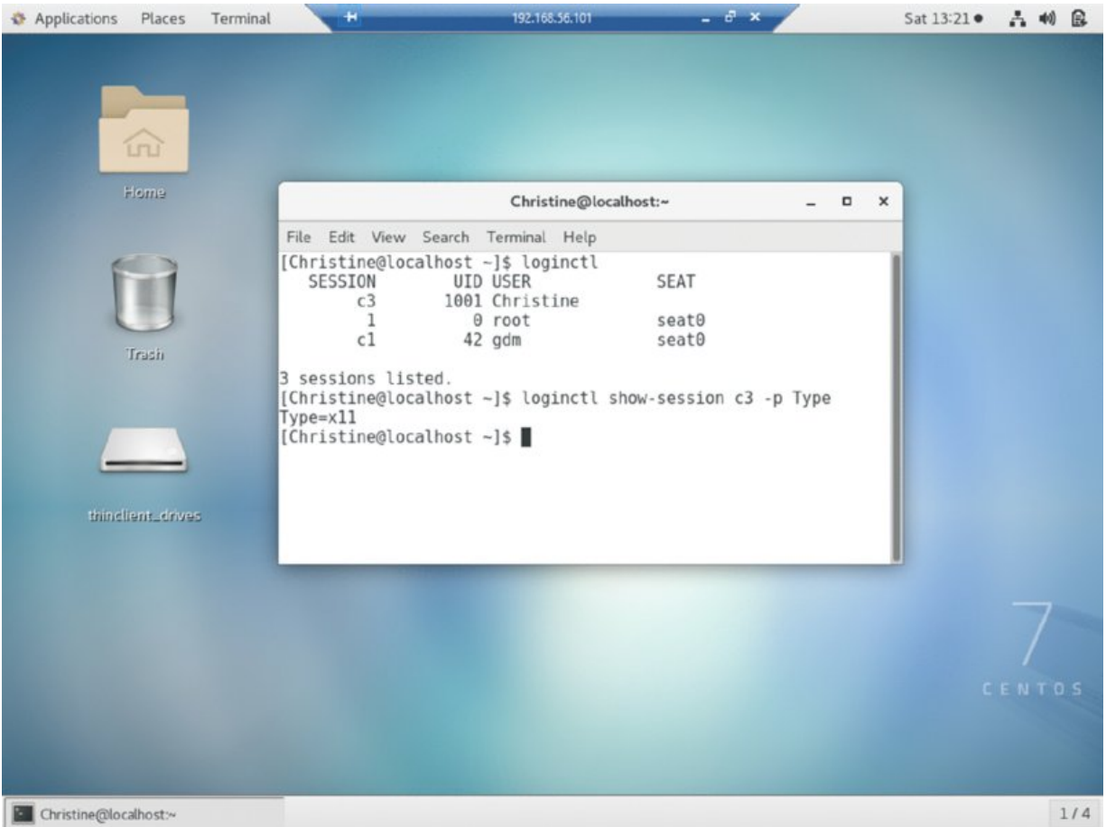
Figure 8.9 Using Xrdp
