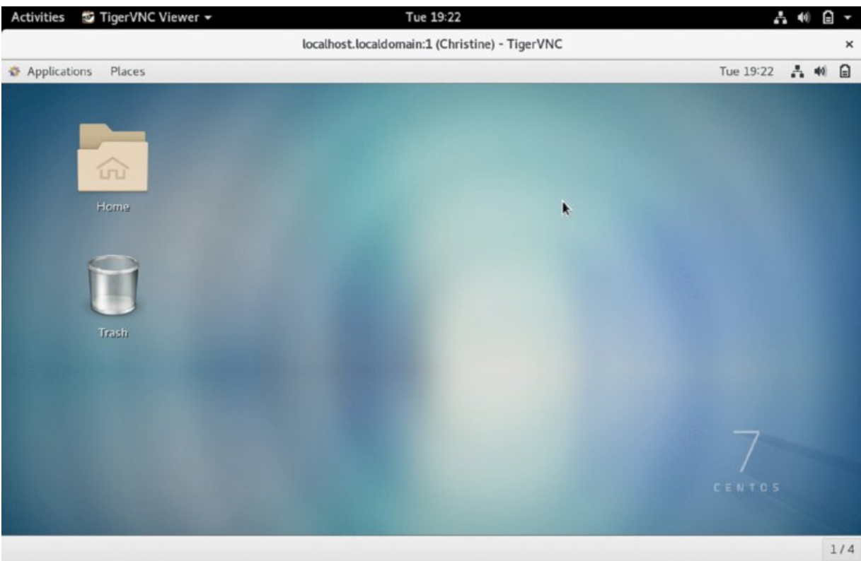
Figure 8.8 Using TigerVNC
