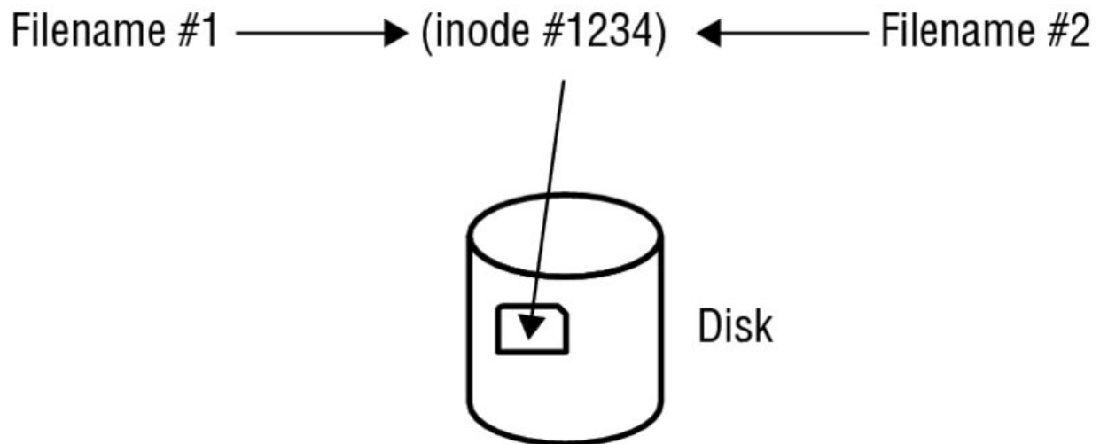
Figure 3.1 Hard link file relationship
