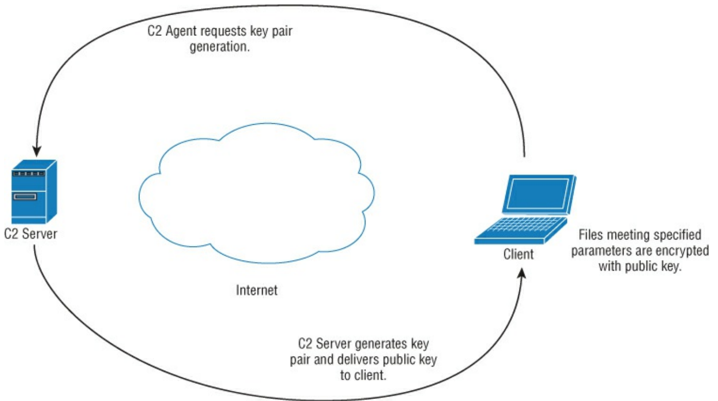
Figure 5.3: Encryption process flow.
