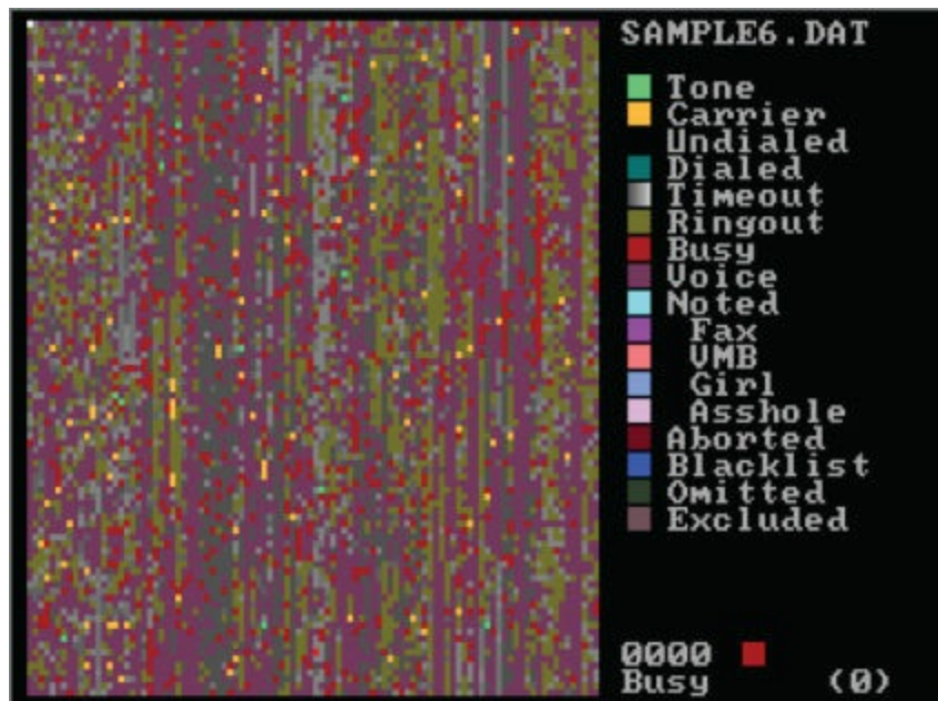
Figure 9.16: Taneloc output.
