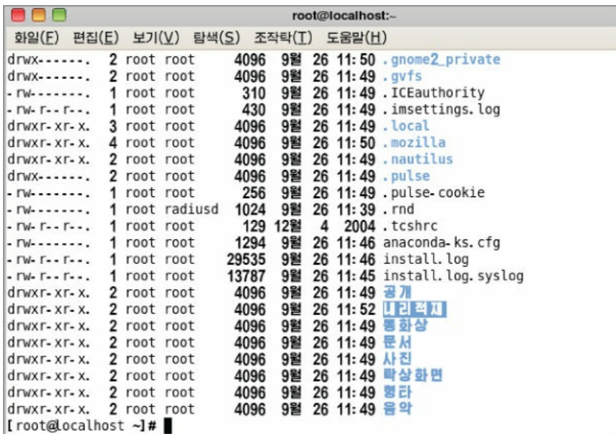
Figure 9.3: A shell.
